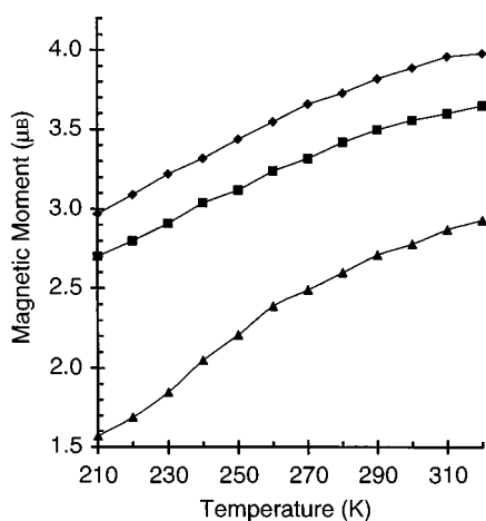
Fig. 4 Temperature-dependent magnetic moment data for [\text{CoL}^1]^{2+}[\text{PF}_6]_2 \cdot \text{H}_2\text{O} ( \blacklozenge ), [\text{CoL}^2]^{2+}[\text{PF}_6]_2 \cdot 2\text{H}_2\text{O} ( \blacksquare ) and [\text{CoL}^3]^{2+}[\text{PF}_6]_2 \cdot 3\text{H}_2\text{O} ( \blacktriangle ) in acetone solution
